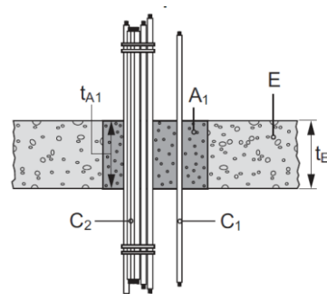
Single cables / cable bundles with additional protection
