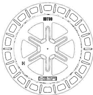
Figure A3: Slip-on plate HDT 90
