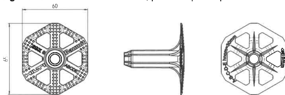
Figure A2: Plate
