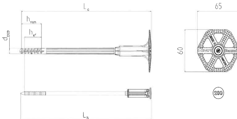
Figure A1: Assembled sleeve, plate and plastic pin
